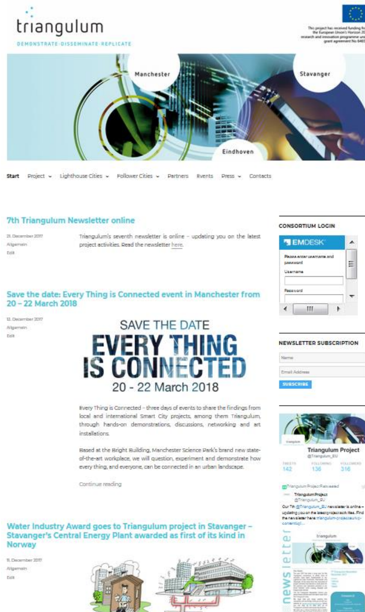
Figure 3: Project Website
